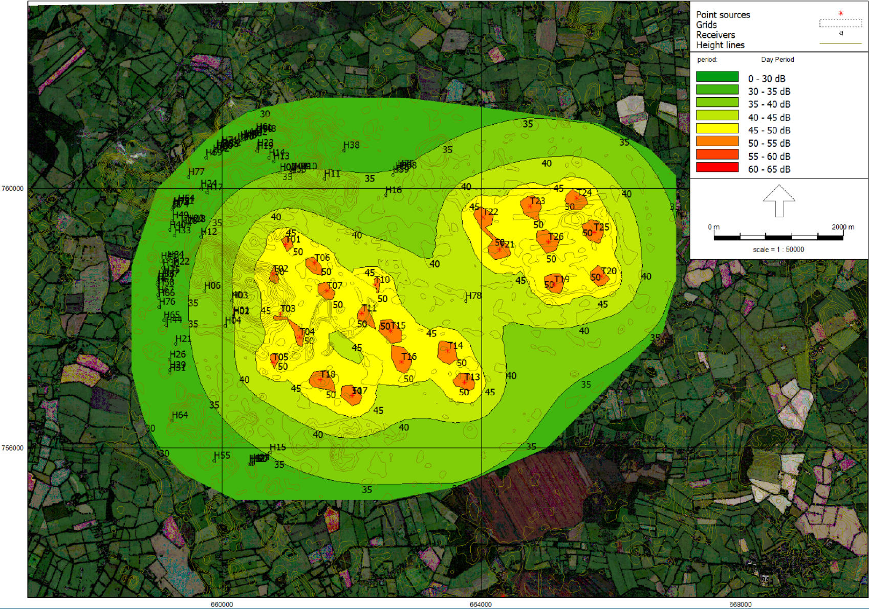
Annex 11.8: Bracklyn Wind Farm Cumulative Noise Contour
